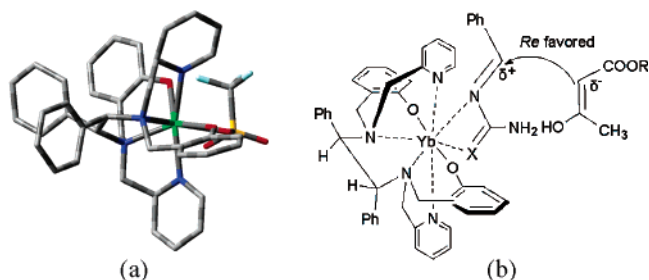
Figure 2. (a) Molecular model of the chiral catalyst Yb-2a. (b) Proposed working model for the asymmetric Biginelli reaction catalyzed by Yb-2a (other groups omitted for clarity).
