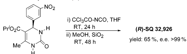
Scheme 2. Synthesis of (R)-SQ 32,926
