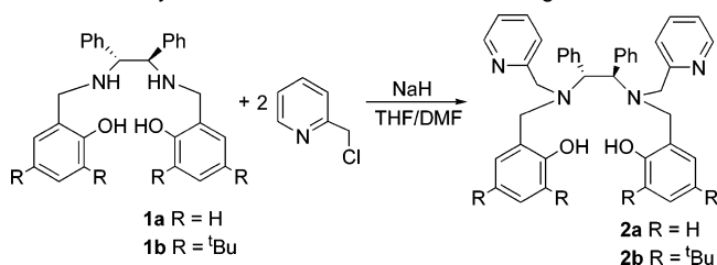
Scheme 1. Synthesis of the Hexadentate Chiral Ligands
